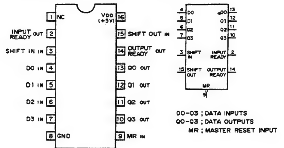
uPD3341C (NEC) N-MOS 256-BIT (64x4) FIRST-IN FIRST-OUT SERIAL MEMORY — TOP VIEW —
